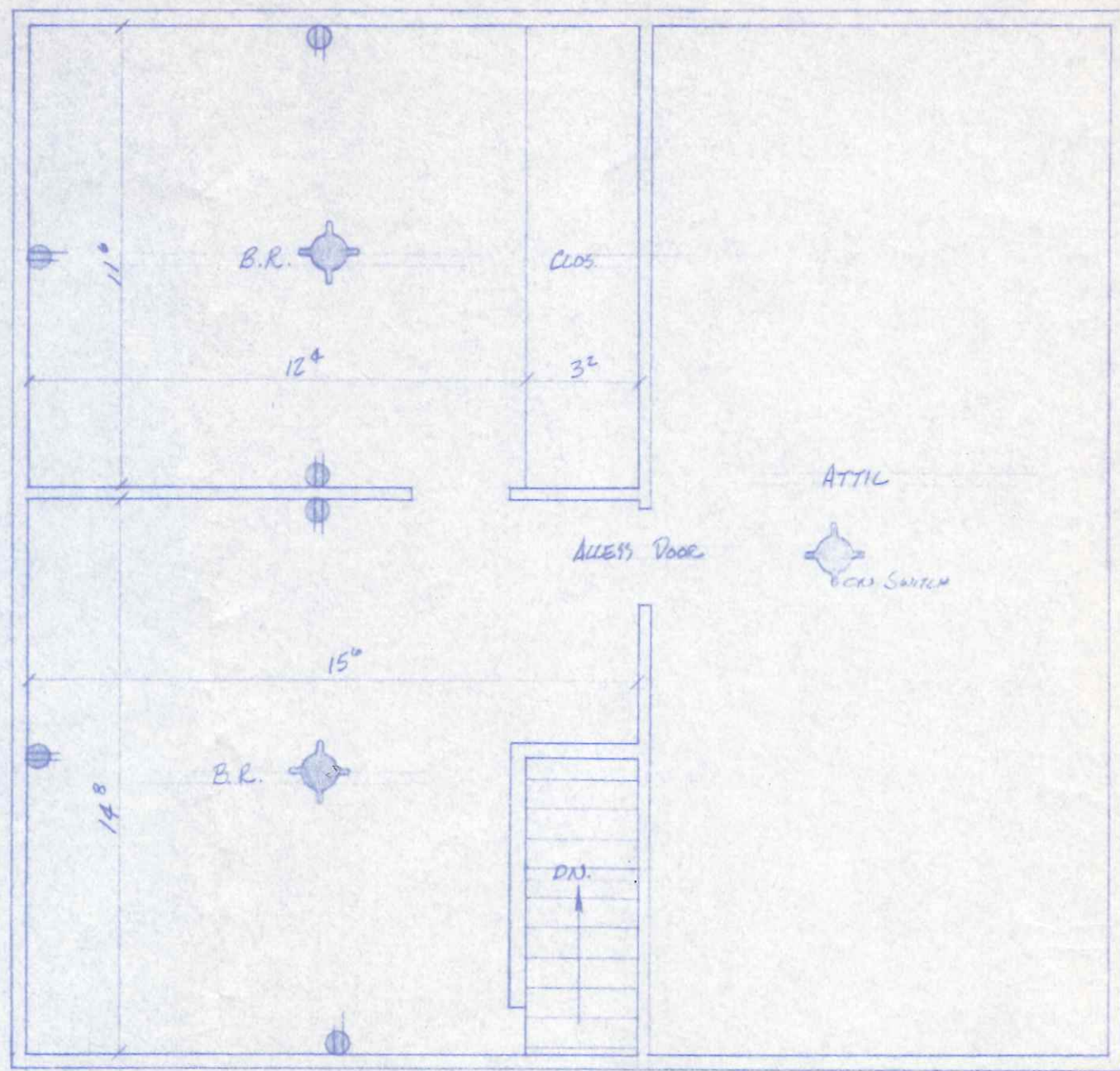
2 ND FLOOR 1/4" = 1'-0"
