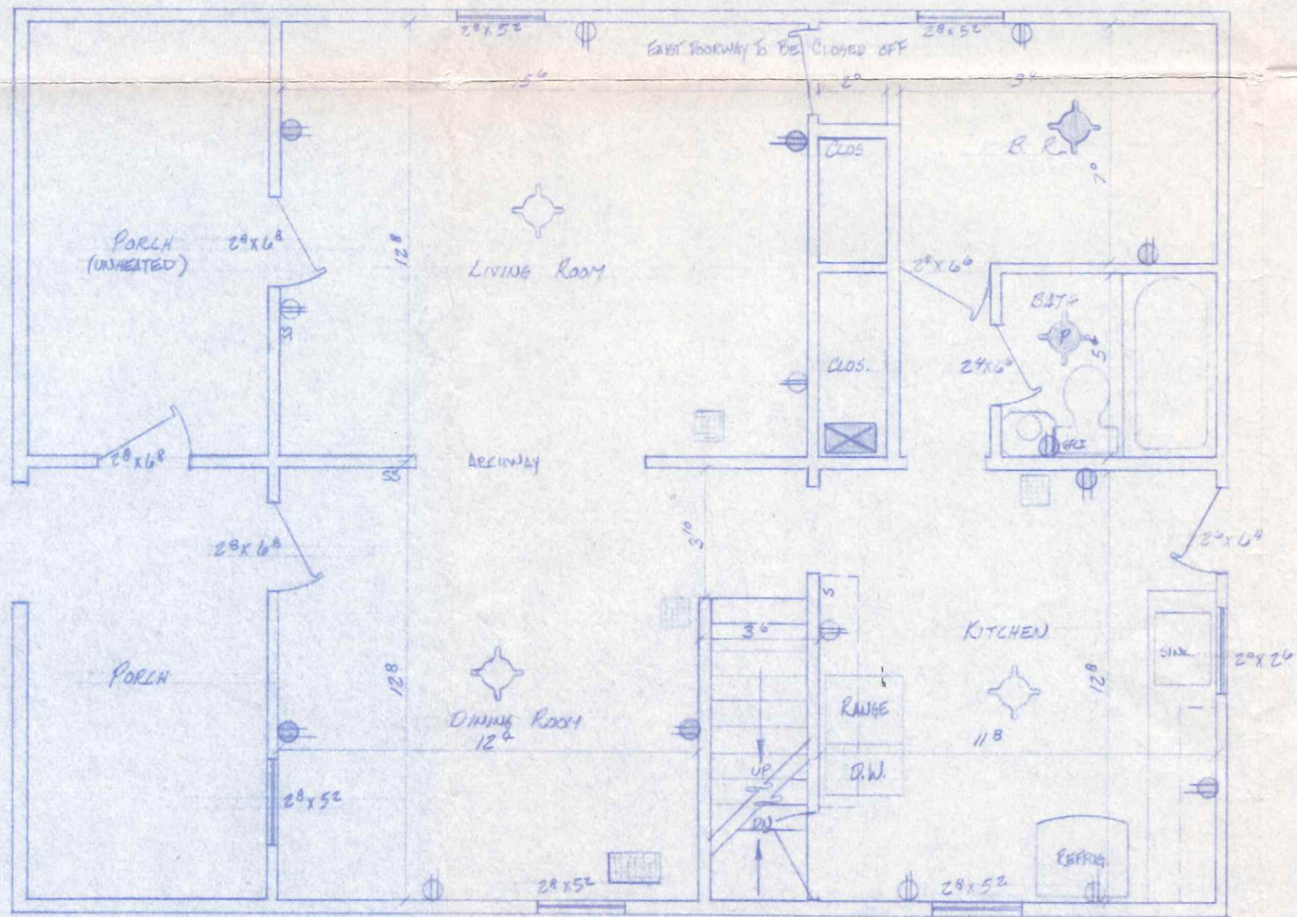
1 ST FLOOR 1/4" = 1'-0"
